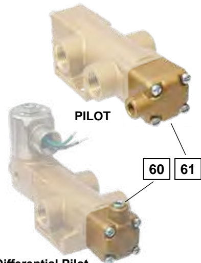
Differential Pilot
